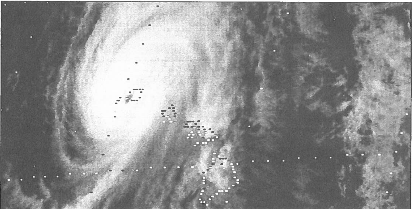
A National Weather Service satellite photo shows the eye of Hurricane Iniki passing directly over Kauai on the afternoon of Sept. 11, 1992.
