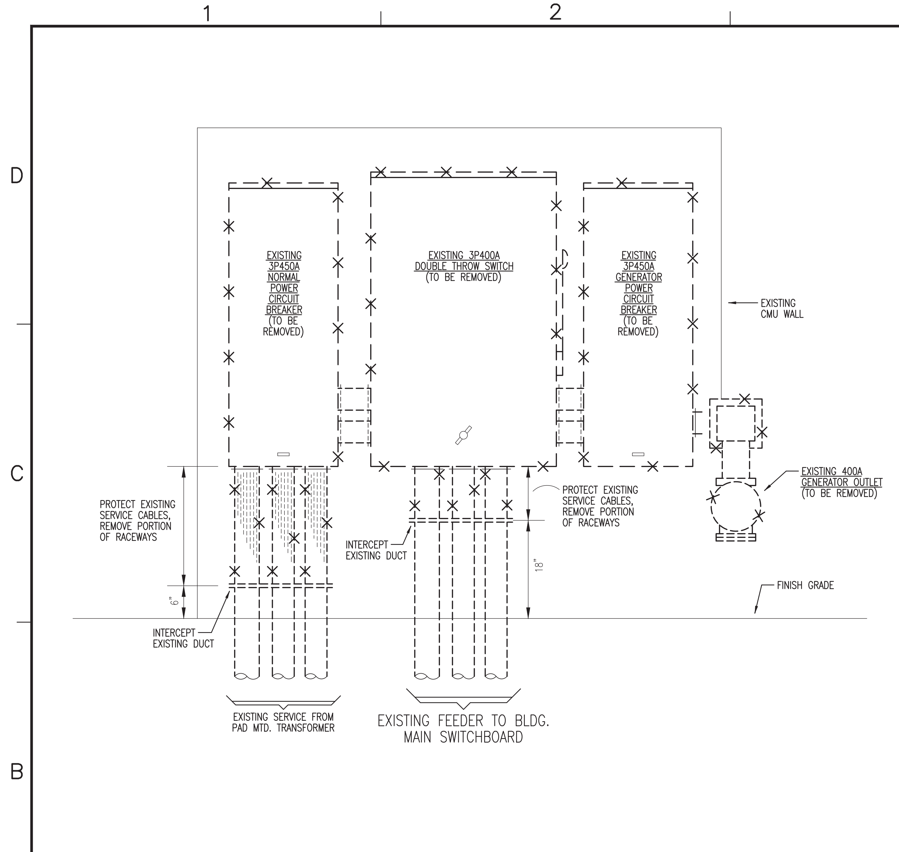
C1 ELEVATION - EXISTING ELECTRICAL SERVICE EQUIPMENT (REMOVAL WORK) NOT TO SCALE
