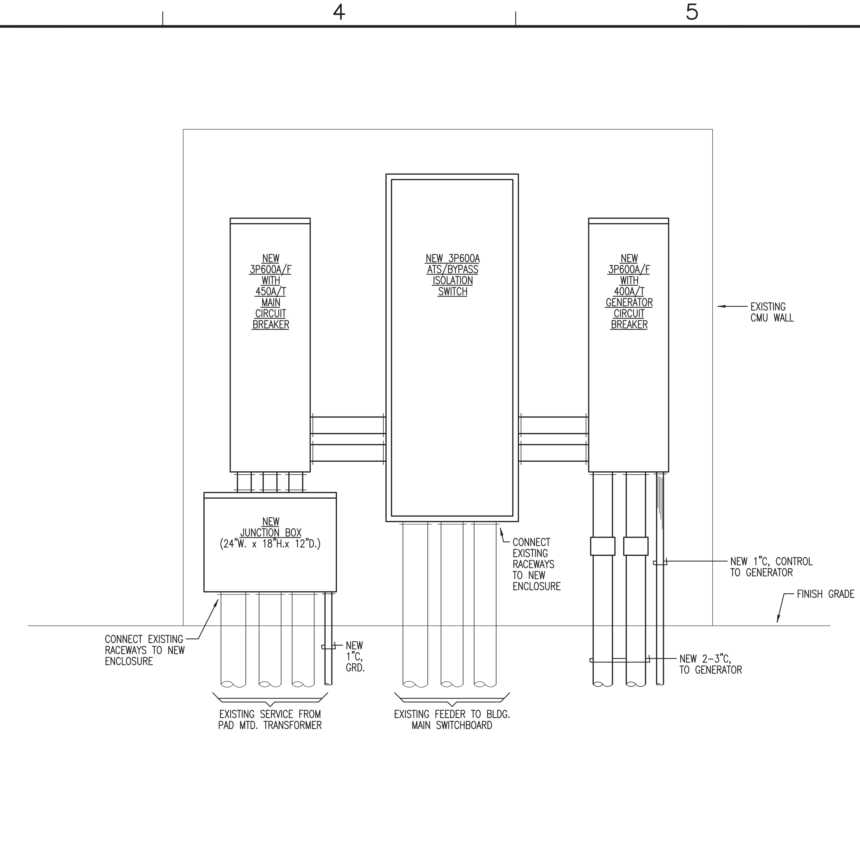
C3 ELEVATION - NEW ELECTRICAL SERVICE EQUIPMENT NOT TO SCALE
