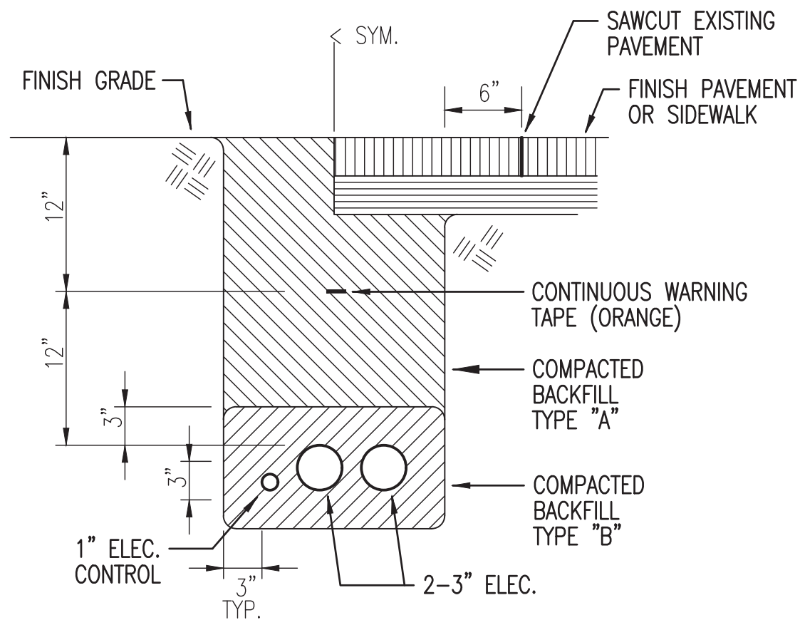
A DUCT SECTION
