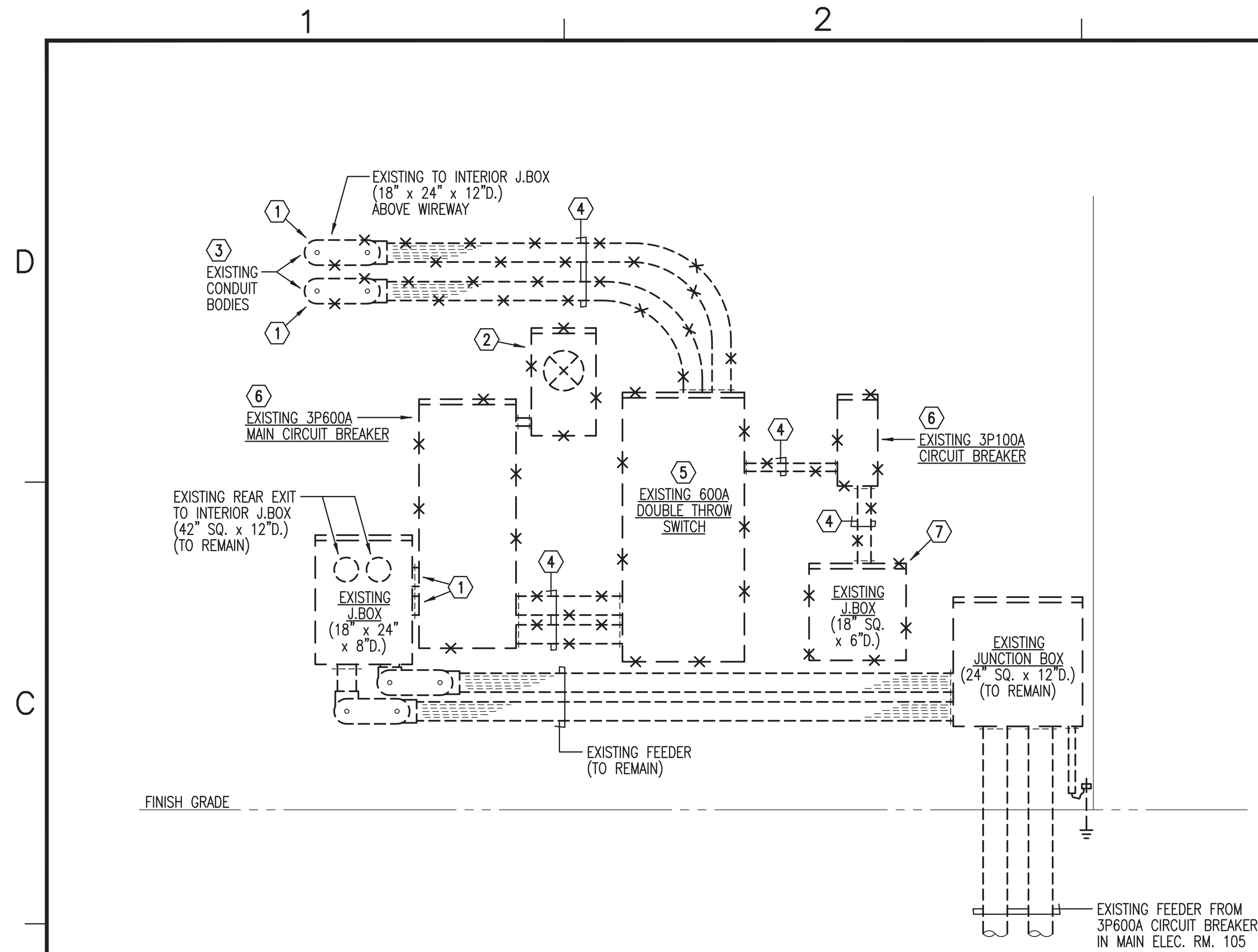
B1 EXTERIOR ELEVATION - MAIN ELECTRIC ROOM 120 (REMOVAL WORK) NOT TO SCALE
