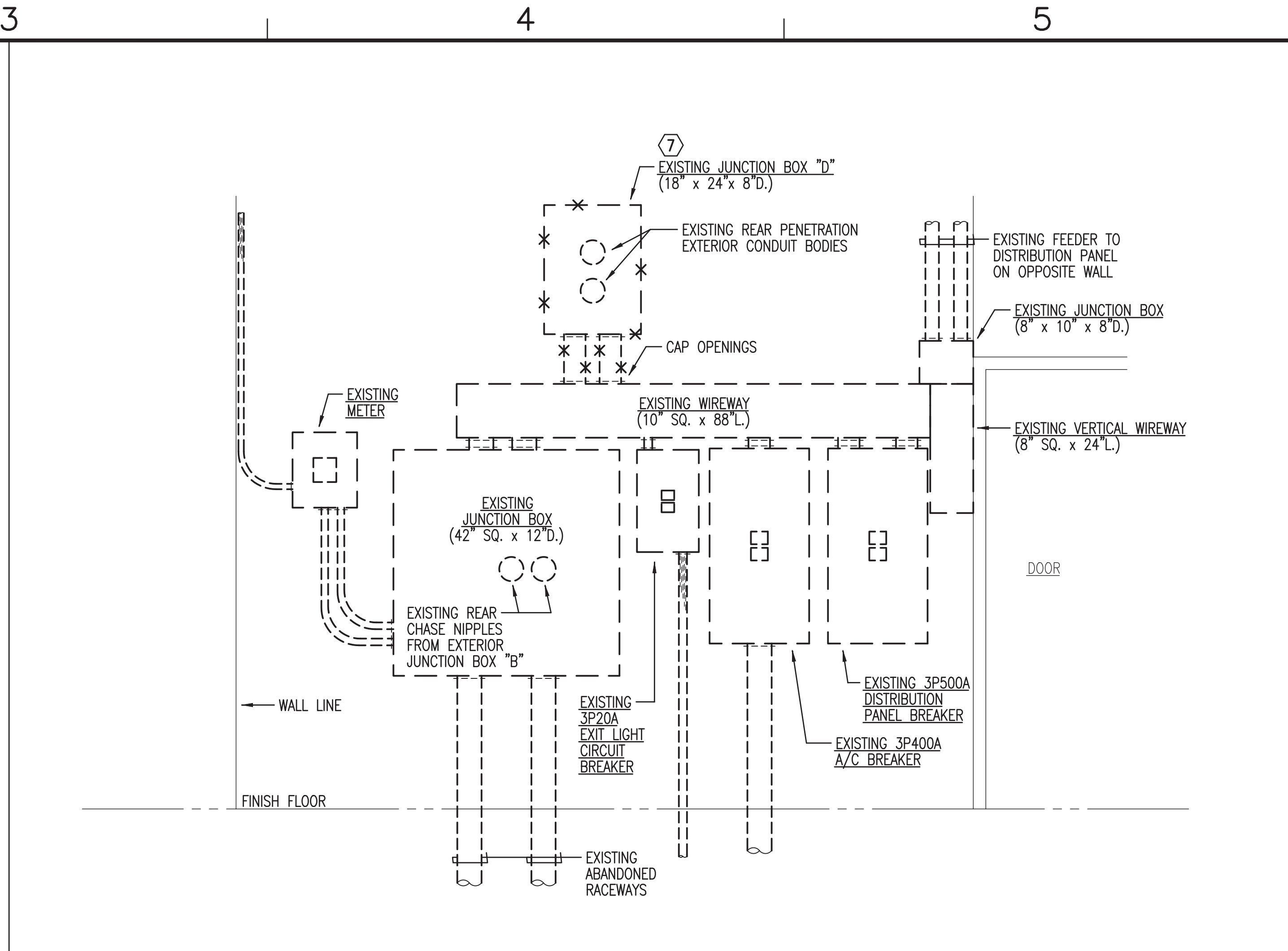
B3 INTERIOR ELEVATION - MAIN ELECTRIC ROOM 120 (REMOVAL WORK) NOT TO SCALE
