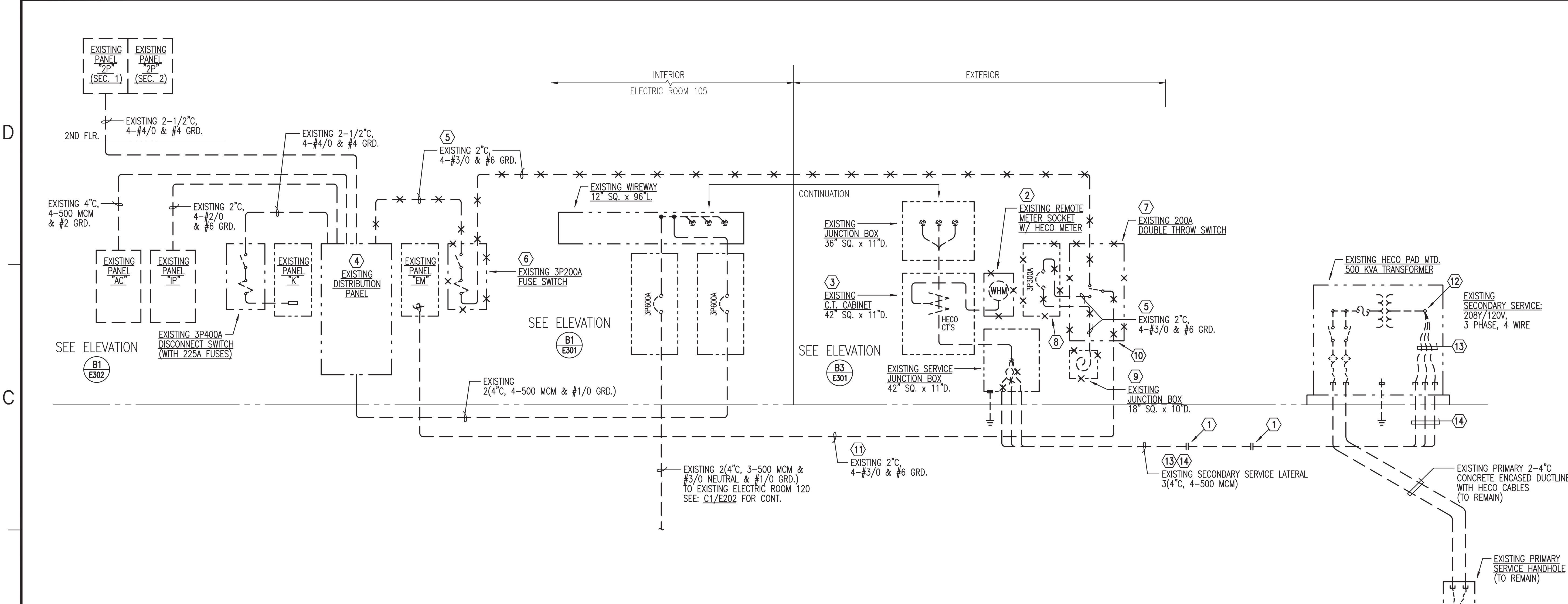
B1 TWO STORY WING - ELECTRIC ROOM 105 - EXISTING ONE LINE DIAGRAM (REMOVAL WORK) NOT TO SCALE
