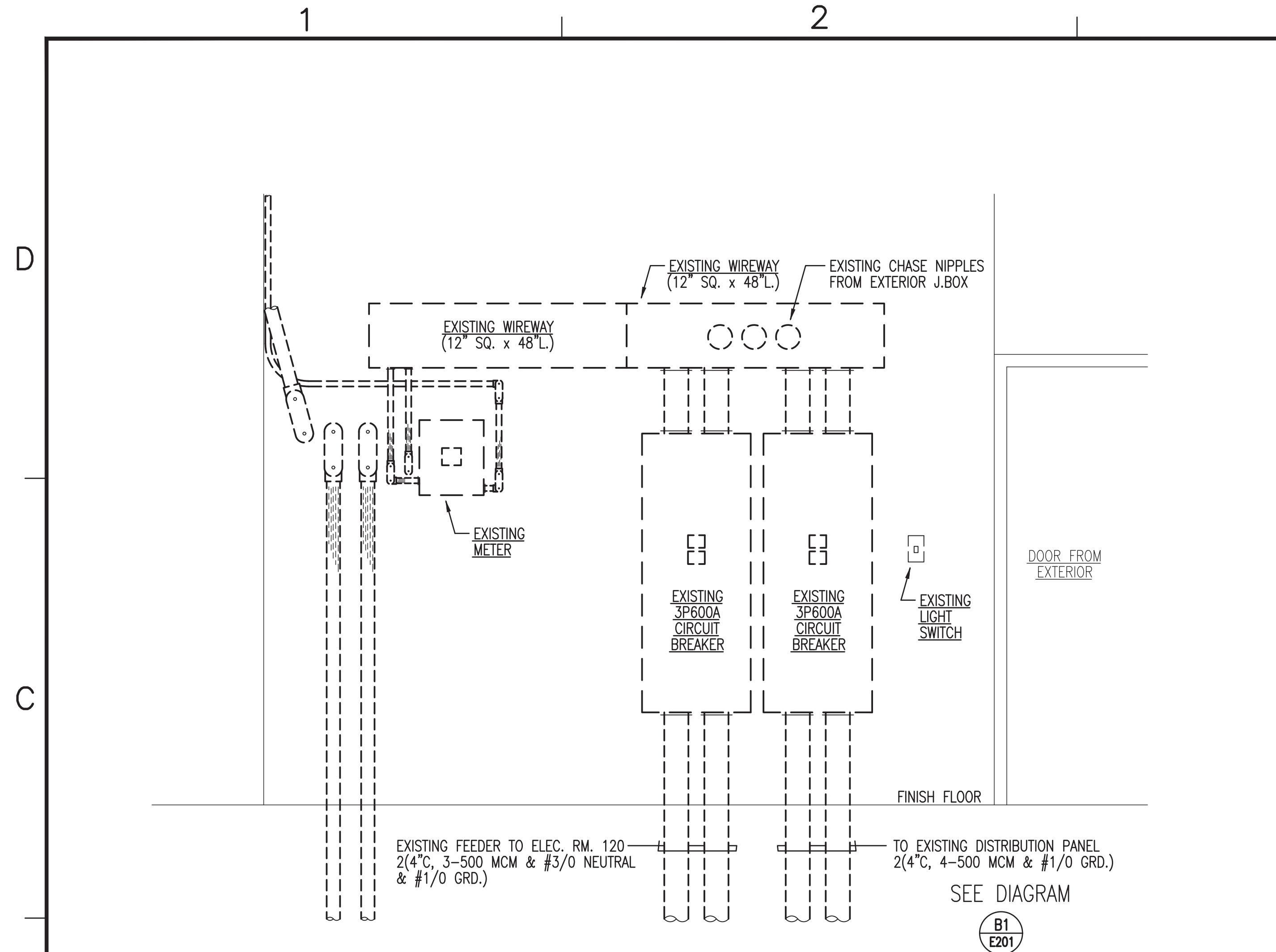
B1 INTERIOR ELEVATION - MAIN ELECTRIC ROOM 105 NOT TO SCALE
