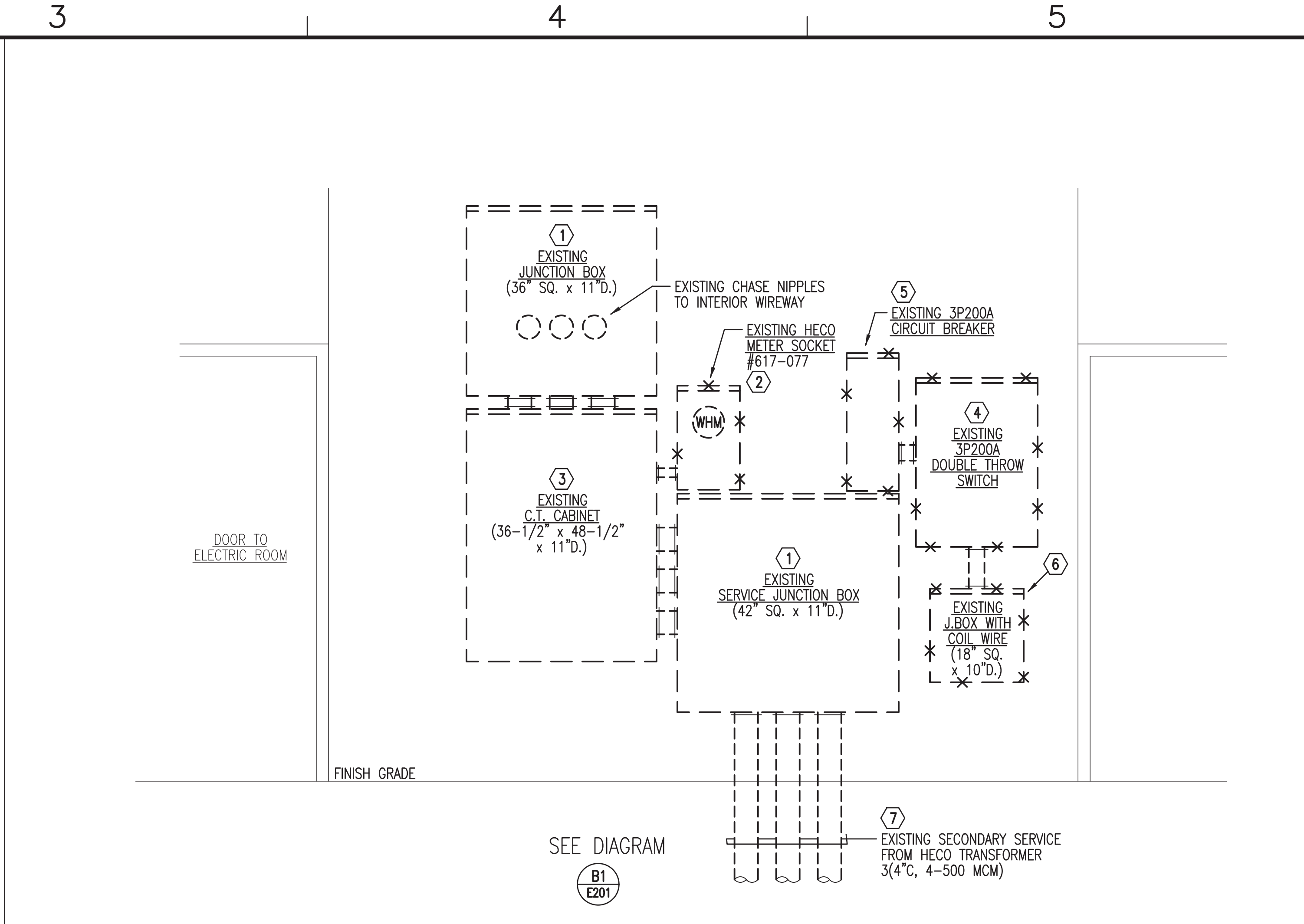
B3 EXTERIOR ELEVATION - MAIN ELECTRIC ROOM 105 (REMOVAL WORK) NOT TO SCALE
