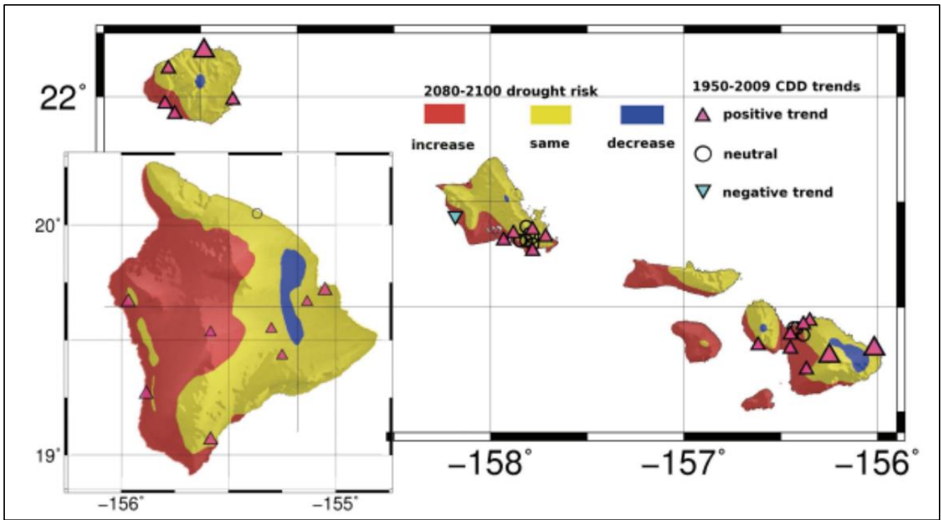
Figure 4.4-8. Future Projections of Drought Based on Historical Data and Future Climate Projections
