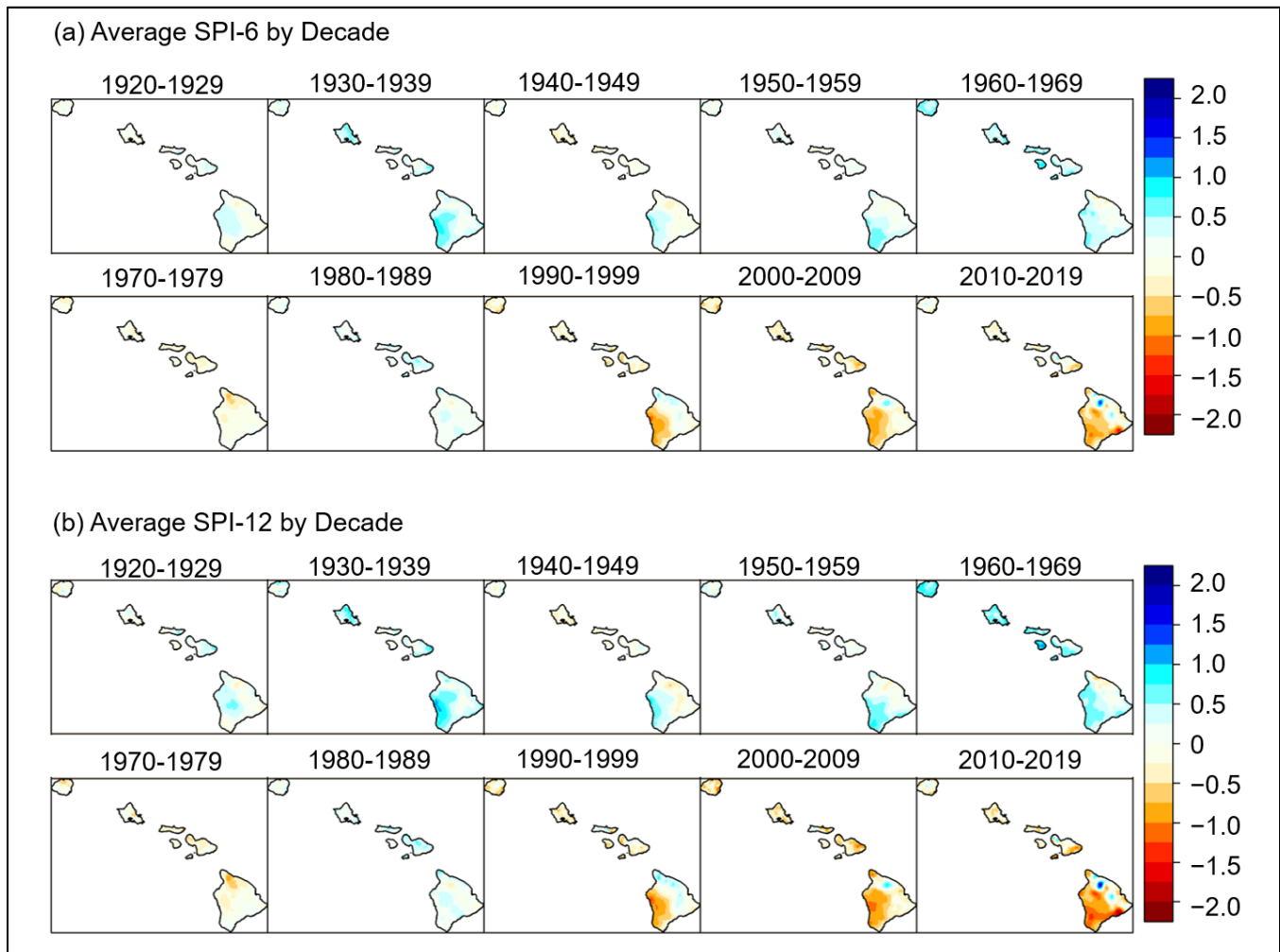
Figure 4.4-6. Average 6-month (a) and 12-month (b) SPI by decade (1920–2019) for the State of Hawai'i
