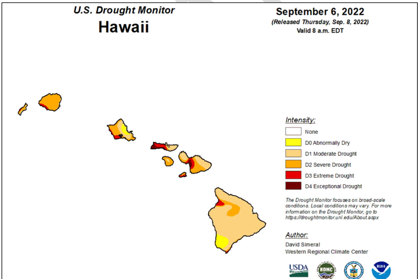
Figure 4.4-2. Drought in Hawai'i, 2022
