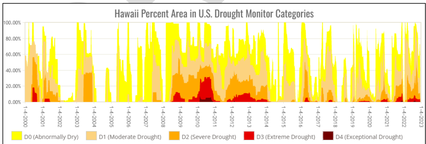
Figure 4.4-7 Percent of Hawai'i State Affected by Each USDM Rating, 2000–2022
