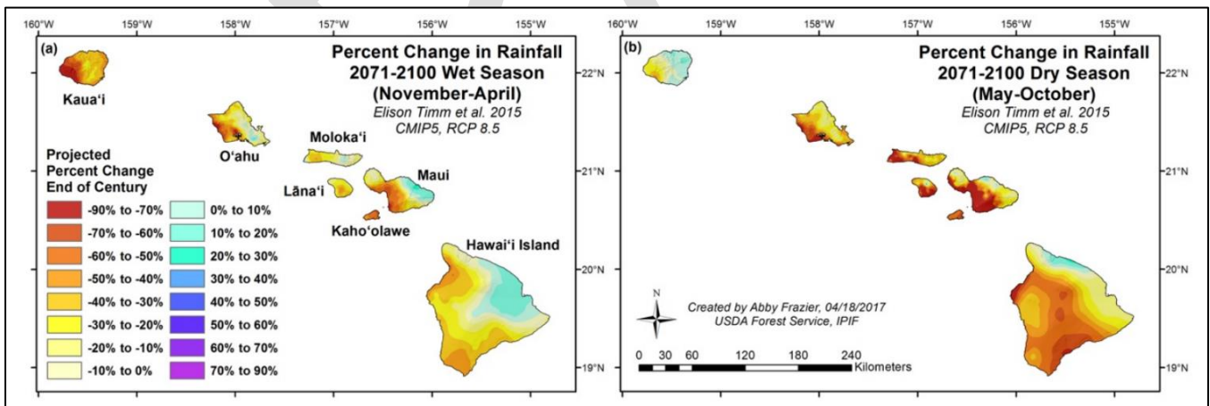
Figure 4.4-9. Percent Change in Rainfall
