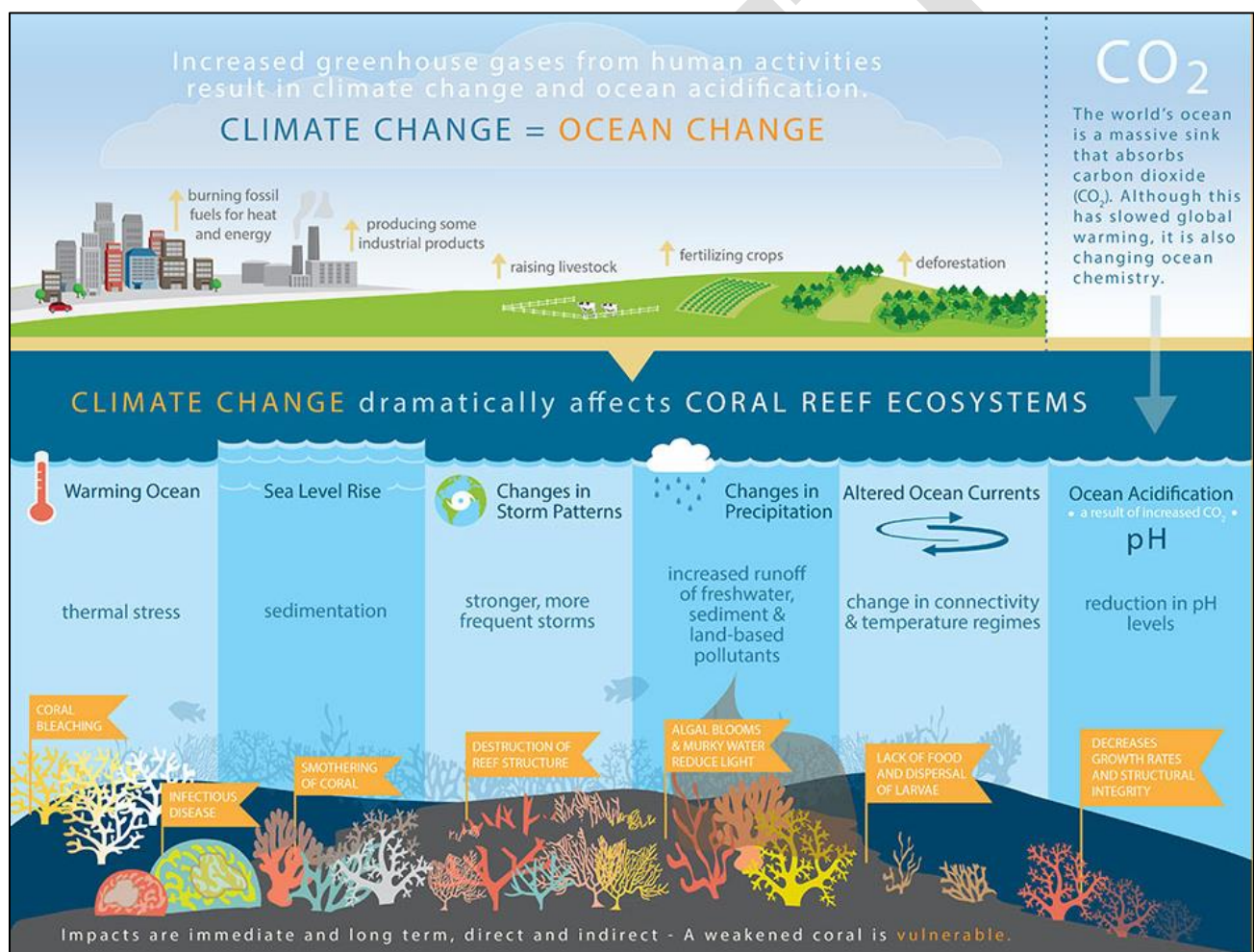
Figure 4.2-12. Climate Change Threats to Coral Reefs
