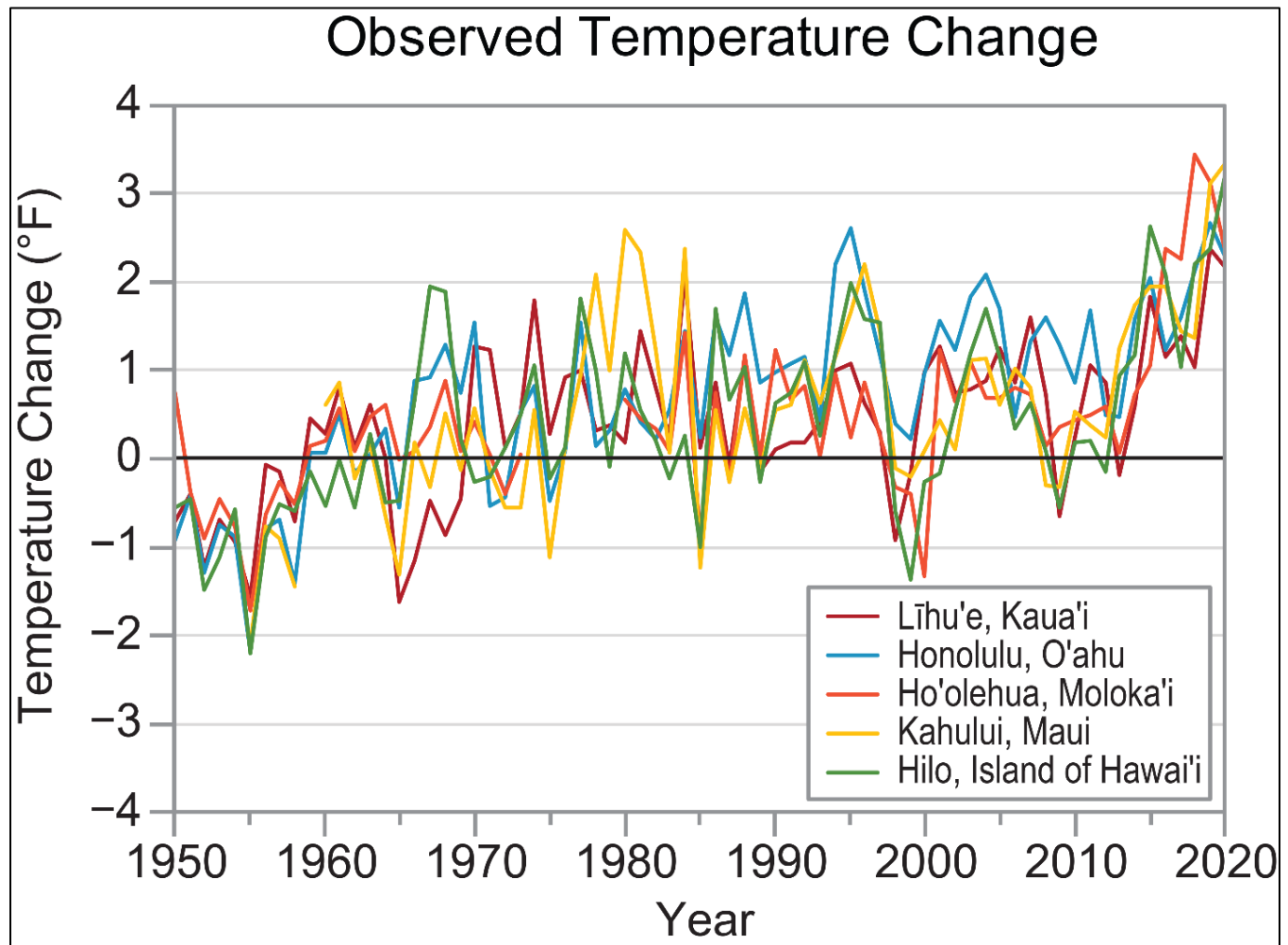
Figure 4.2-2. Observed Hawai'i Temperature Change
