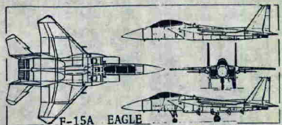
F-15A EAGLE
